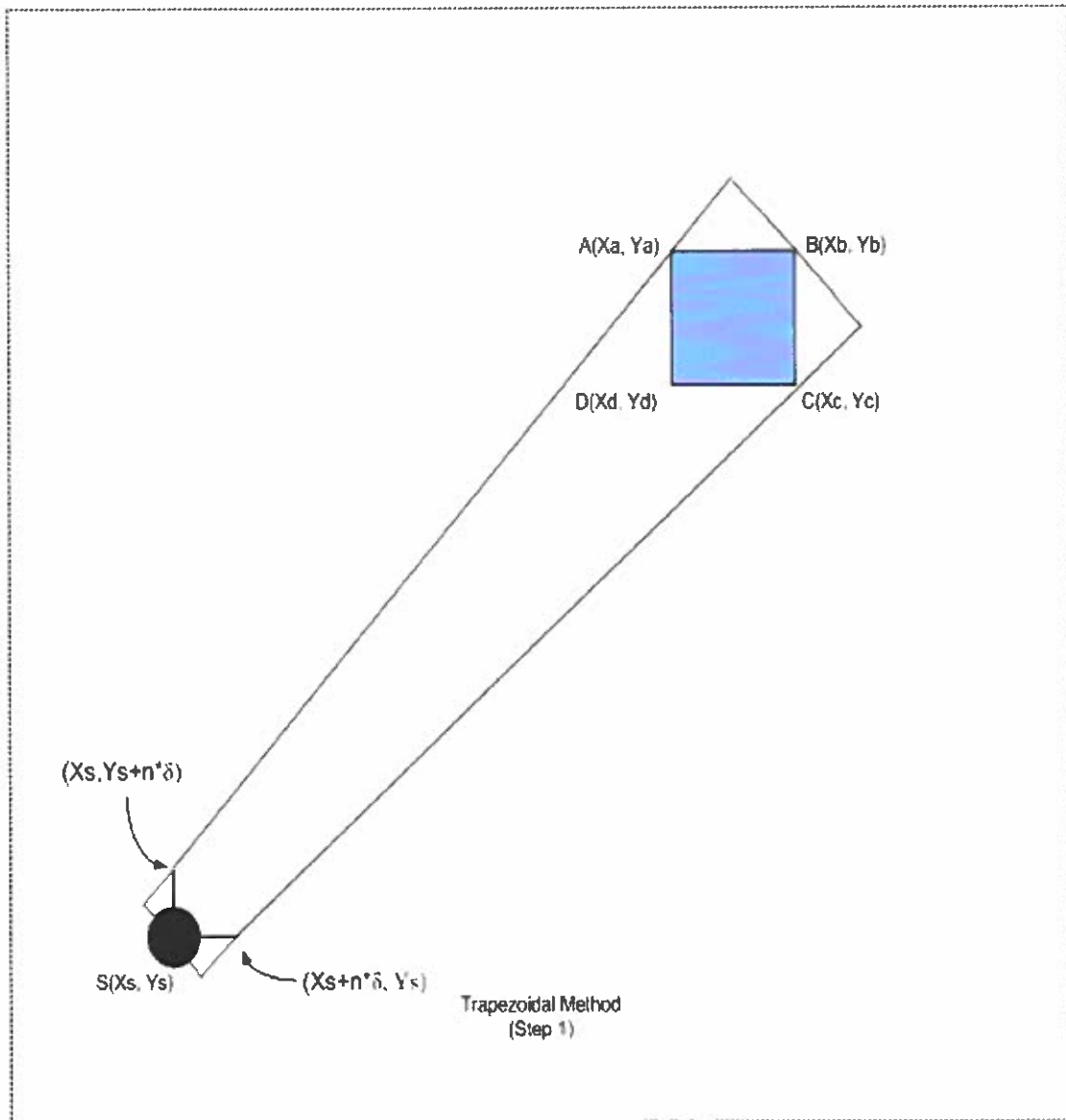
Figure 9: 1 st step of the Trapezoidal Method
